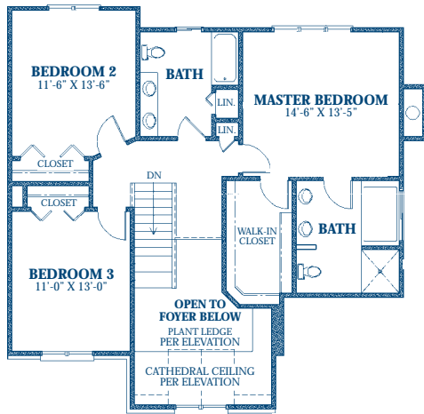
Second Floor 3 Bedroom
